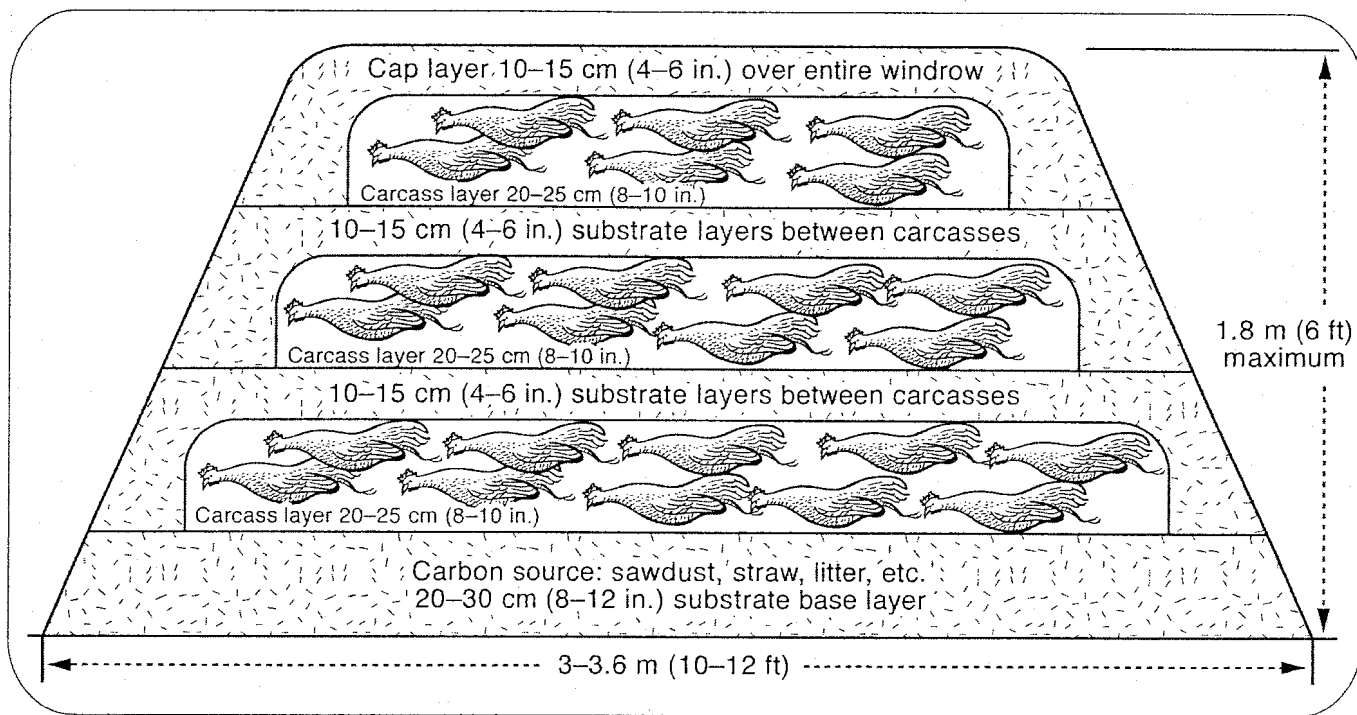
Figure 2. Cross-section of a carcass-composting windrow created using the layering method.
