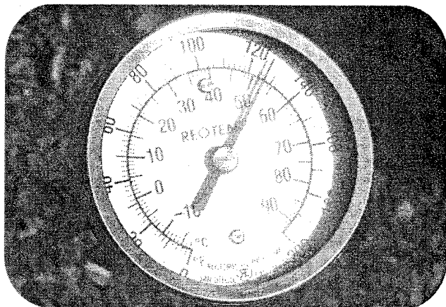
Figure 3. Long-stem thermometer inserted in compost pile recording a temperature of 51°C (124°F).
