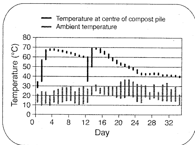
Figure 4. Time versus temperature graph of a compost windrow. The pile was turned at Day 13.
